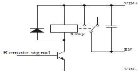
Transistor control
