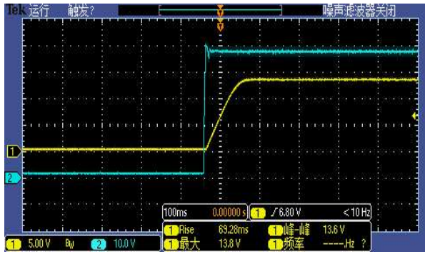
Figure 6, Output voltage established (Iout = 20A)
