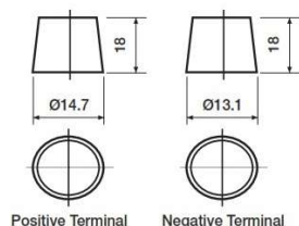
Positive Terminal
